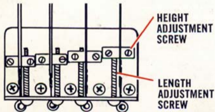
FIGURE 2 BRIDGE
